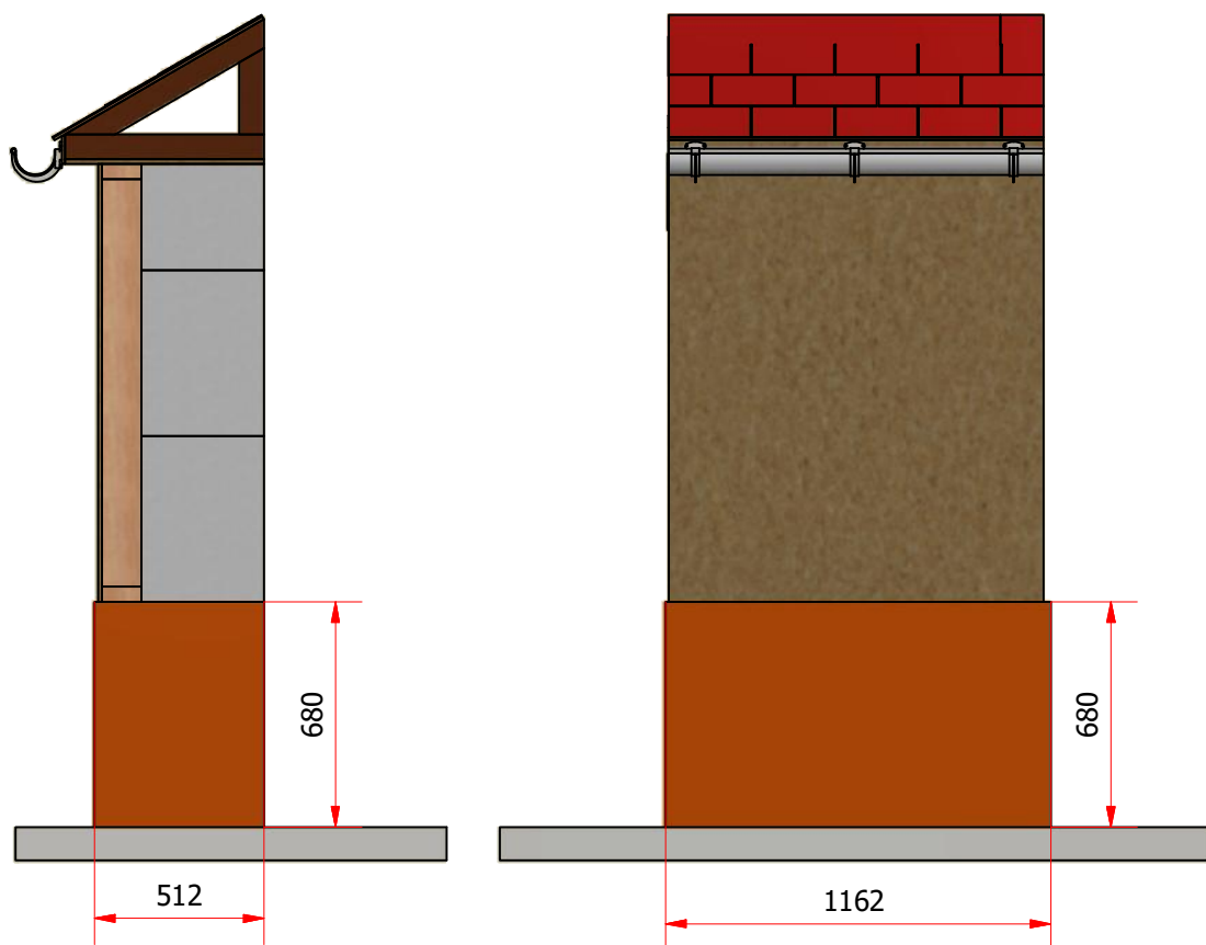
FACADE ( 1 :25 )
